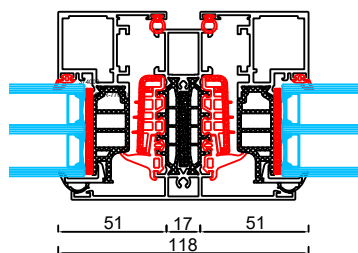
4 fixed mullion
