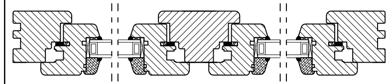
Horizontal Cross-section
