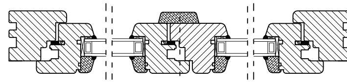
Horizontal Cross-section
