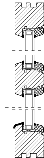
Vertical Cross-section
