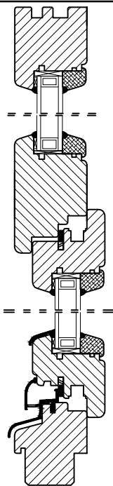
Vertical Cross-section
