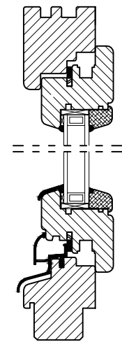
Vertical Cross-section
