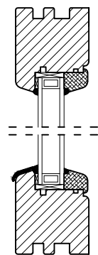
Vertical Cross-section
