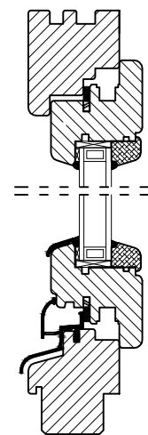
Vertical Cross-section
