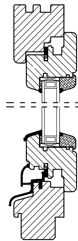
Vertical Cross-section
