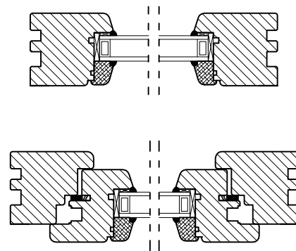
Horizontal Cross-section
