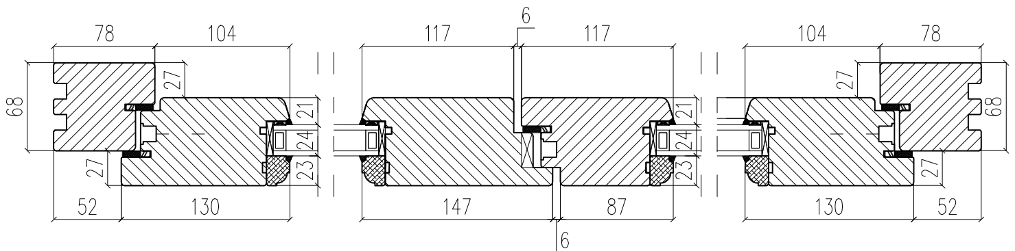
B - B Horizontal cross-section
